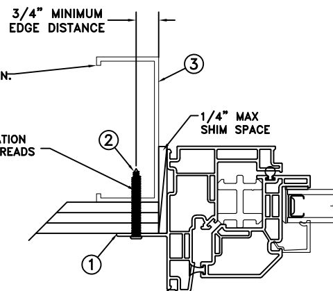
FRAME JAMB SECTION (TYP) HORIZONTAL SECTION
