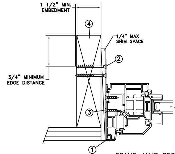
FRAME JAMB SECTION (TYP) HORIZONTAL SECTION
